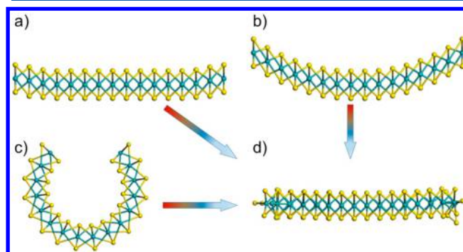
Figure 6. (a–c) initial (deformed) and (d) final (optimized) structures of MoS 2 nanomesh.
