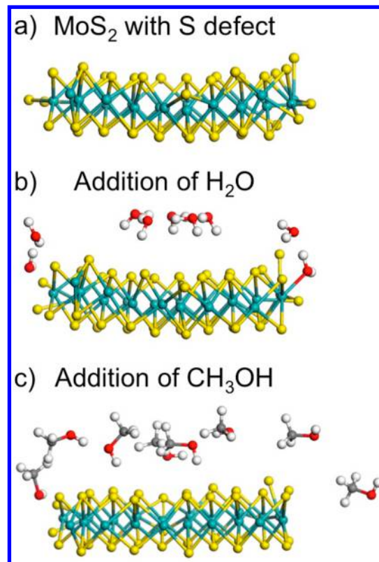
Figure 8. Optimized structures of MoS 2 nanomesh with a single sulfur defect (a) in vacuum, (b) with surrounding H 2 O molecules, and (c) with surrounding CH 3 OH molecules.
