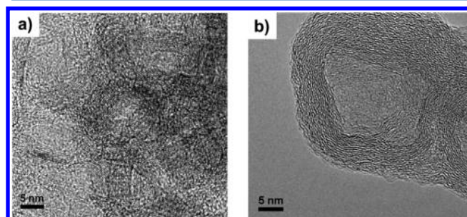
Figure 4. HRTEM images of 3D MoS 2 NS and zoom of single isolated 3D MoS 2 nanosheet showing fullerene-like structure.
