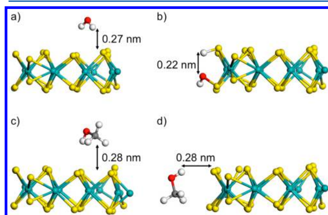
Figure 7. Single H 2 O molecule (a) adsorption on surface (b) and dissociation at the edge; and single CH 3 OH molecule adsorption (c) on surface (d) at the edge of MoS 2 nanomesh.
