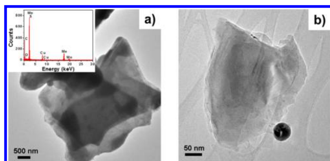
Figure 3. Representative TEM images of the MoS 2 NS indicating multilayer and few NS by the PLA of bulk MoS 2 powder in methanol. Inset, EDS spectrum.
