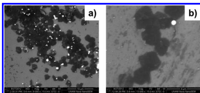
Figure 2. Representative SEM images of MoS 2 NS obtained by PLA in an organic liquid. SEM images confirm 2D MoS 2 NS and 3D MoS 2 NS production in one step.
