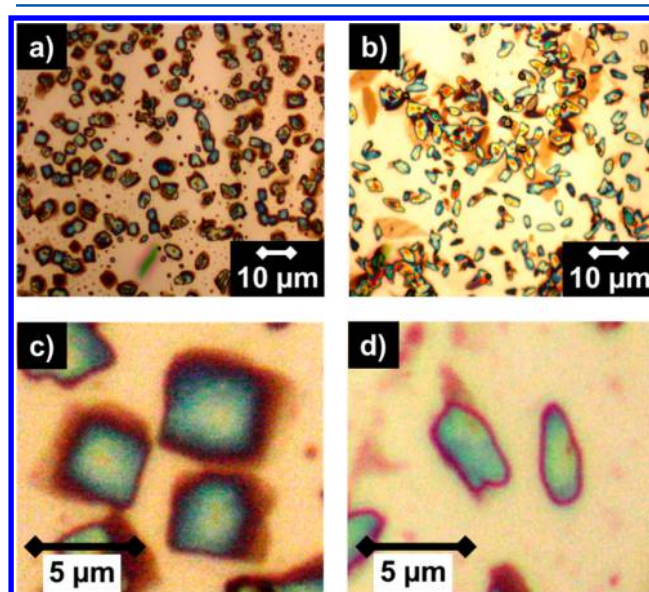
Figure 1. Optical microscope images of MoS 2 NS showing micrometer size layered morphology on a silicon substrate.
